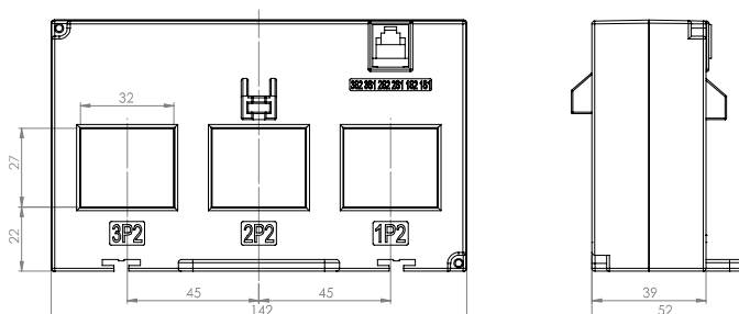
Three-phase transformer RJ12 - busbar 32 x 27 mm
