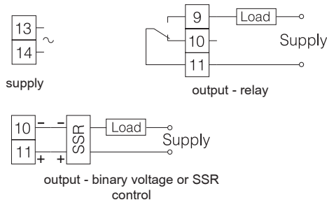
Fig.2. Connection of supply and load circuit.
