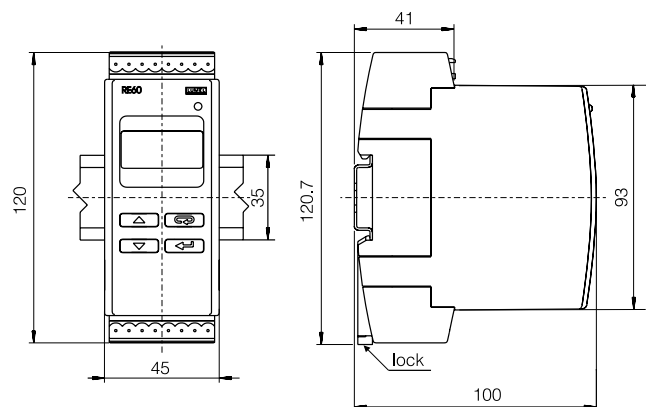
Fig. 1. Dimensions and fixing way of the controller
