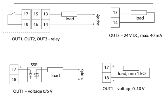
Fig. 3 Connection of steering/alarm outputs
