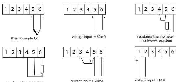
Fig. 2 Connection of measuring signals
