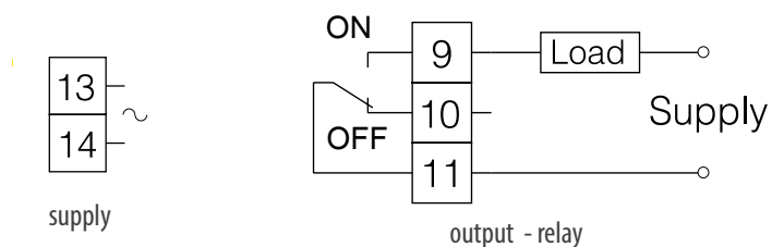
Fig.2. Connection of supply and i load circuit.
