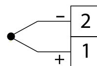
thermocouple
