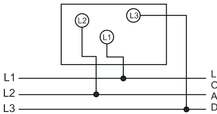
Voltage measurement in 3-phase 3-wire network
