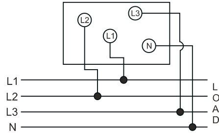
Voltage measurement in 3-phase 4-wire network
