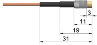
T05-G-KA-VK10 Material: 1.4404
